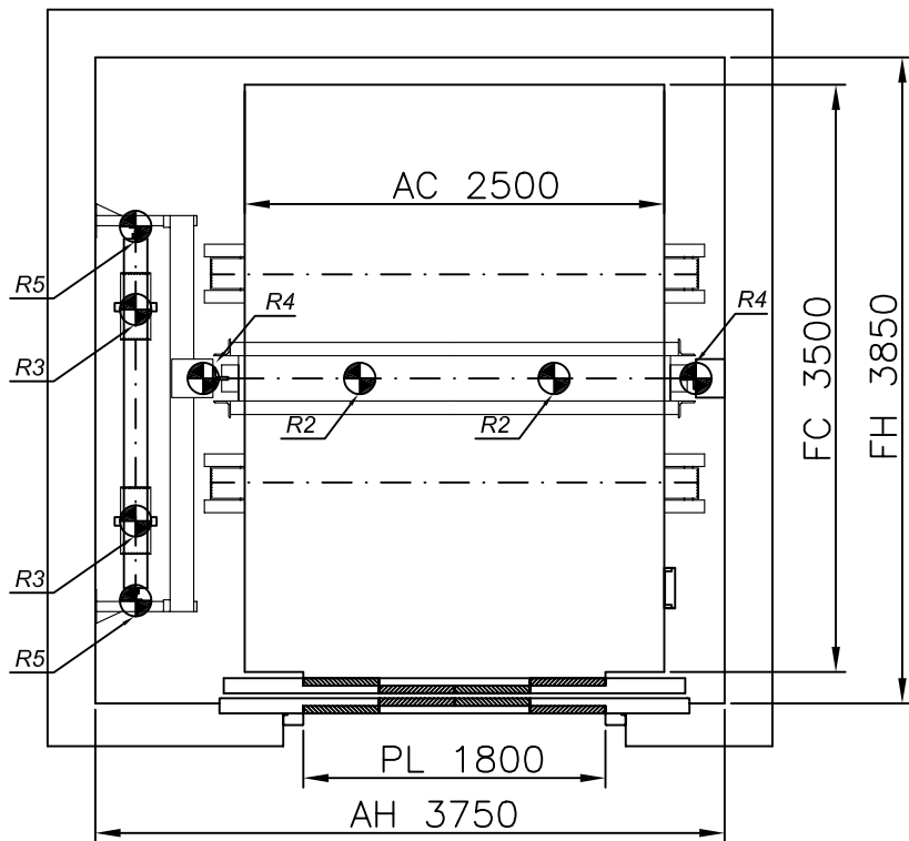
ESCALA/SCALE 1:50
