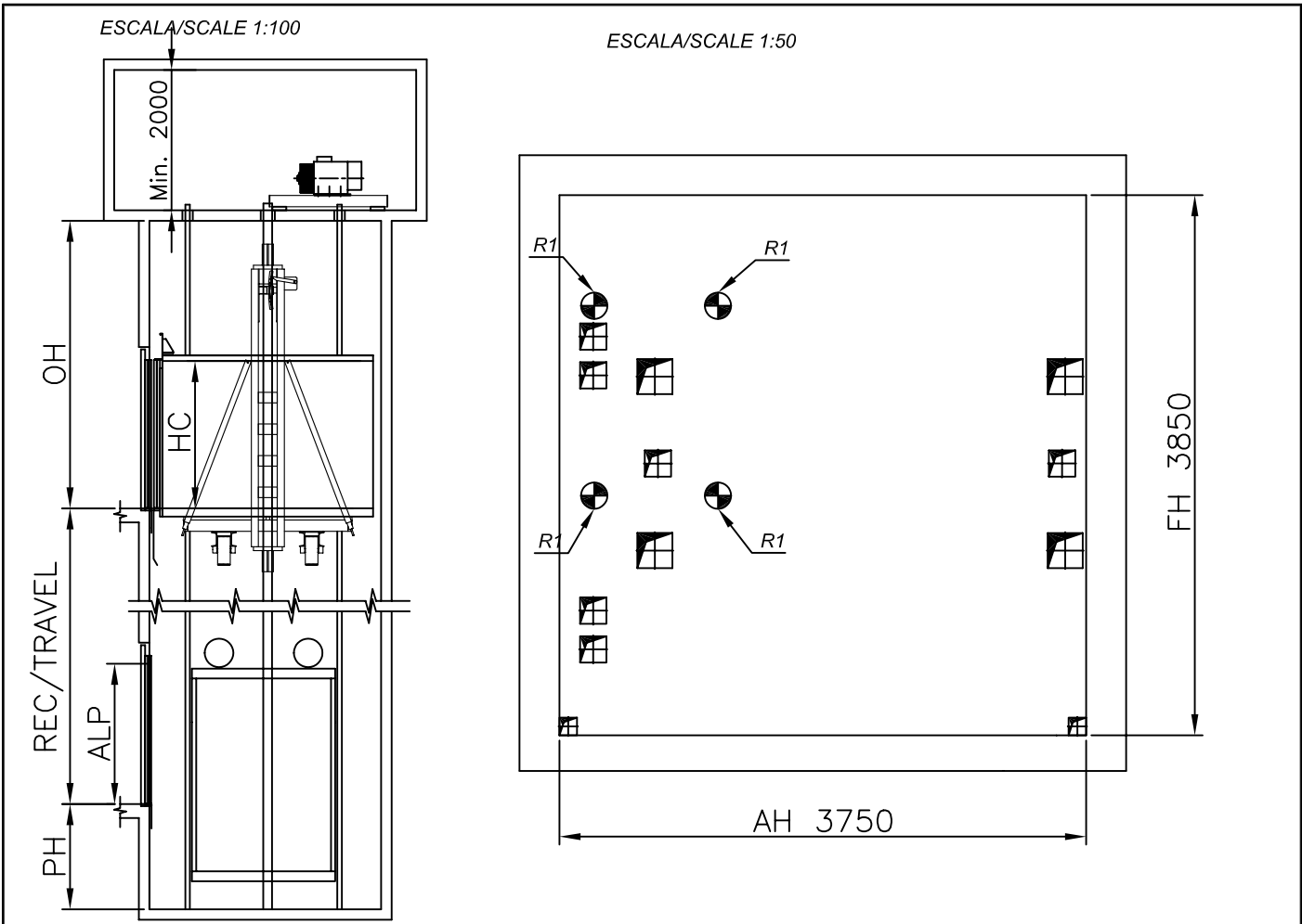
ESCALA/SCALE 1:50
