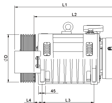
Rolle Ø320/Ø400
